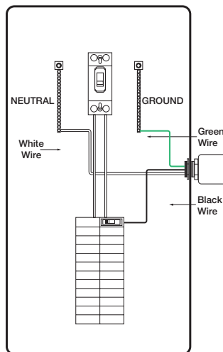
120*240*277*480 VAC Diagram
