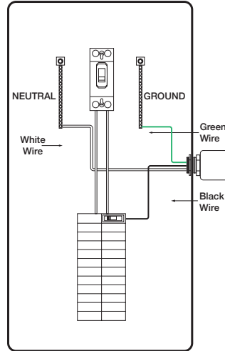
120*240*277*480 VAC Diagram
