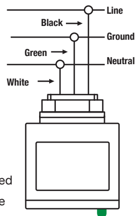
120*240*277*480 VAC Diagram
