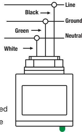
120*240*277*480 VAC Diagram
