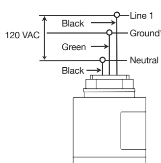
120 VAC Installation
