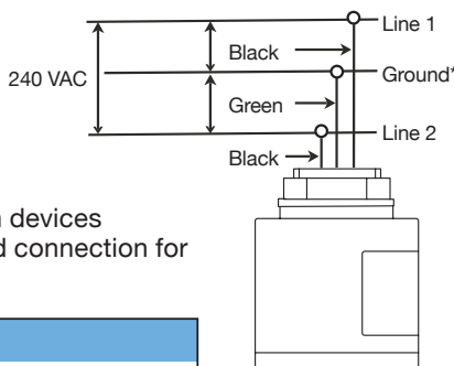
120/240 VAC Installation
